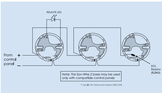
Wiring diagram of Sav-Wire Base
